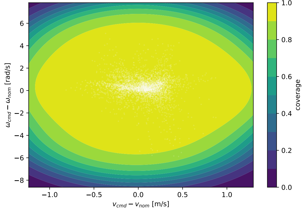
Residual coverage vs command offset (0 = off / OOD; state fixed at mean [0.76 m/s, 0.32 rad/s])
